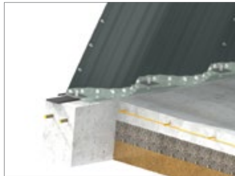
ARCHWALL 4500 FOOTING RENDERING
