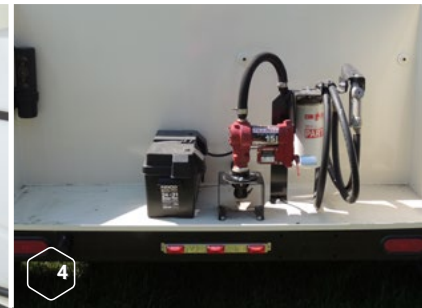
12V Fill Rite Pump, Filter, Hose & Nozzle
